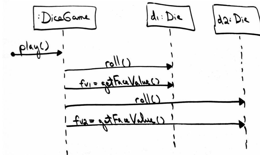
Figure 1.4 Sequence diagram illustrating messages between software objects.
